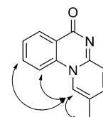
Scheme 3. Identification of the angular isomer 5e by NOESY correlations.
